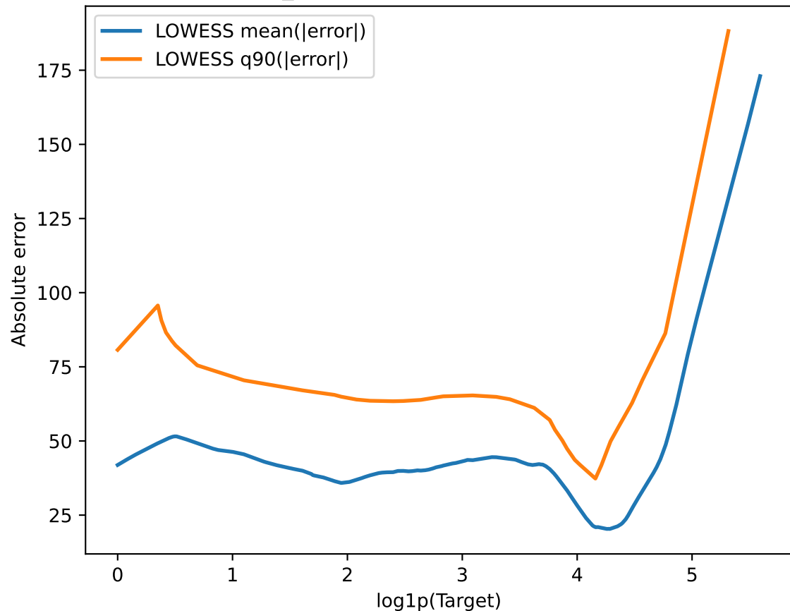
BPIC15_1: Residual trend vs log1p(Target)
